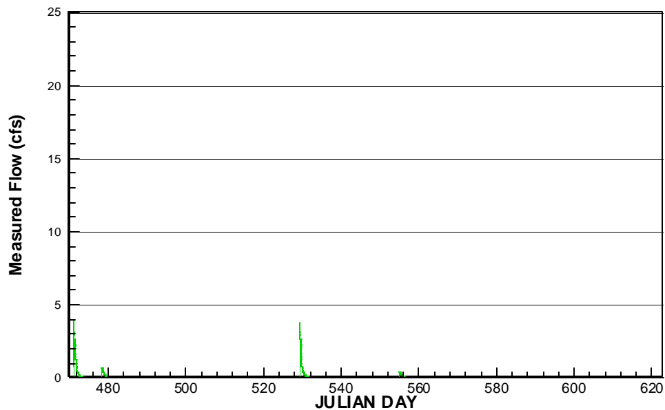
Figure C-7. 15-Minute Measured Flow for Summer 1997 at Station F181-R
