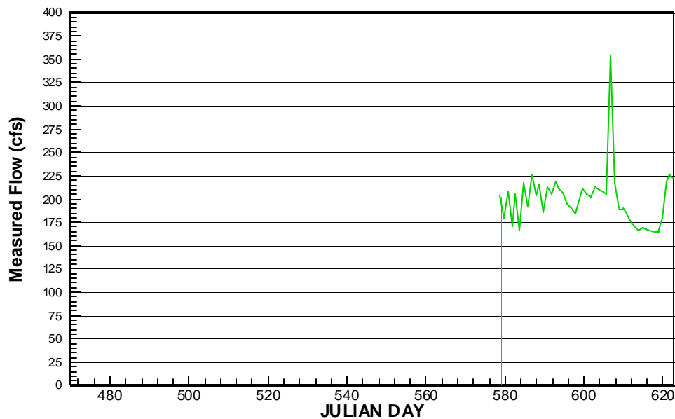
Figure C-18. Daily Averaged Measured Flow for Summer 2000 at Station F319-R
