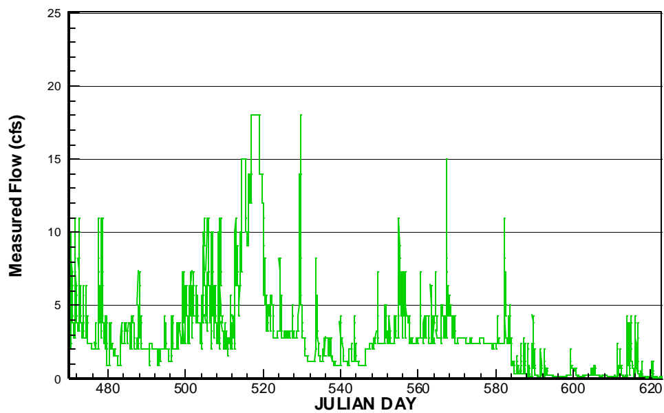
Figure C-8. 15-Minute Measured Flow for Summer 1997 at Station F45B-R
