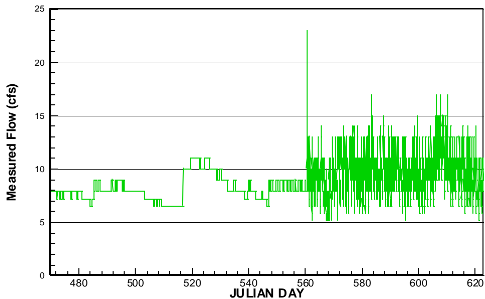
Figure C-3. 15-Minute Measured Flow for Summer 1997 at Station F285-R
