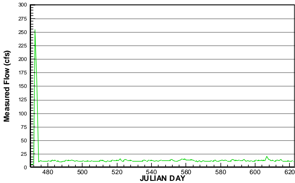
Figure C-16. Daily Averaged Measured Flow for Summer 2000 at Station F285-R
