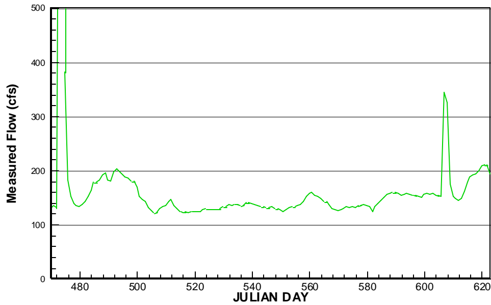
Figure C-12. Daily Averaged Measured Flow for Summer 2000 at Station F34D-R
