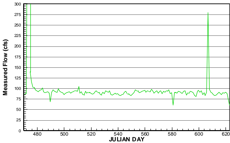
Figure C-17. Daily Averaged Measured Flow for Summer 2000 at Station F300-R
