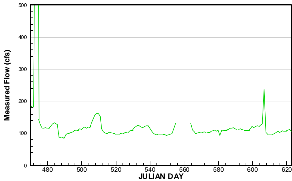
Figure C-13. Daily Averaged Measured Flow for Summer 2000 at Station F57C-R
