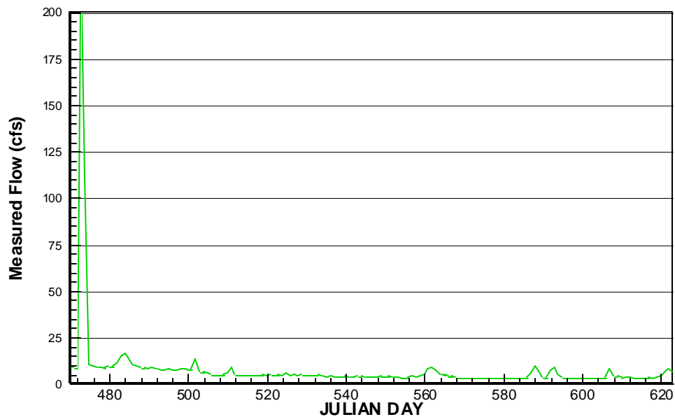
Figure C-14. Daily Averaged Measured Flow for Summer 2000 at Station F252-R
