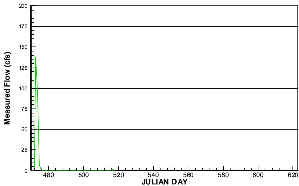
Figure C-15. Daily Averaged Measured Flow for Summer 2000 at Station F277-R
